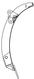
Standard Moldboard vs 12" Extension on Integral Shield Moldboard
