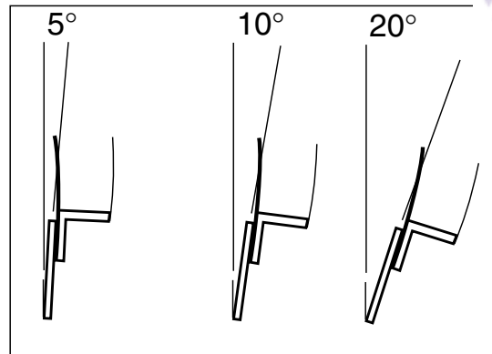
Force Required to Trip Moldboard
