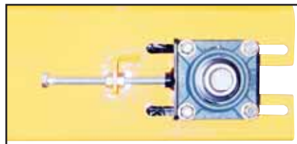
Slotted front longsills for easy removal of chain sprocket assembly.
