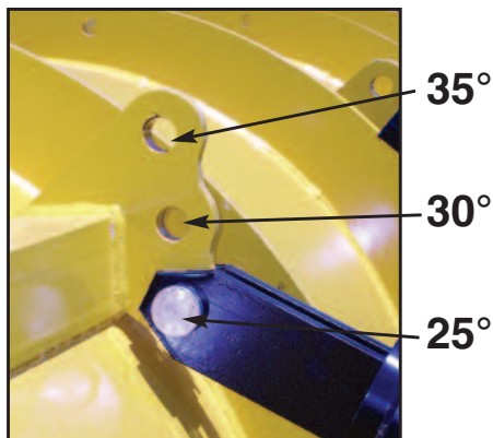
Simple Three Position Adjustment for Plow Cutting Edge Attack Angle
